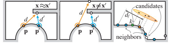
Figure 3: To estimate the correlation in visibility between \mathbf{p} and its neighbor \mathbf{p}' we sample directions and evaluate if the respective distances project to the same (left) or different (middle) surface points. The right image shows the placement of a new cache record.
