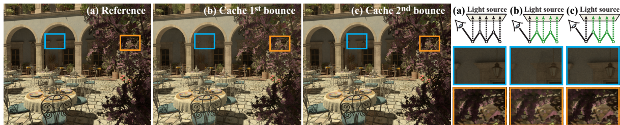
Figure 1: Our visibility caching significantly speeds up tracing of secondary rays, here from 0.15 MRays/s (reference) to 0.70 MRays/s (with the visibility cache). The images were rendered using path tracing where some of the rays (highlighted by green in the illustrations; solid and dashed lines represent path segments and shadow rays, resp.) were traced using our visibility cache with 2000 shadow maps achieving 4.7× higher throughput of secondary rays per second.
